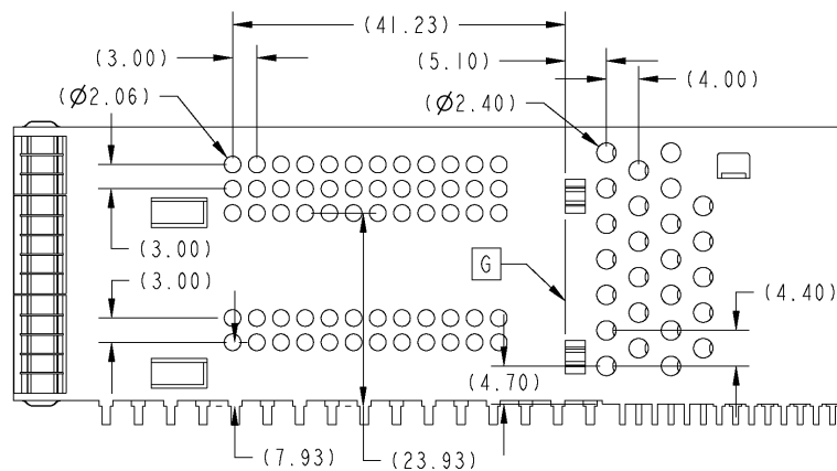
Figure 7-22: Side ventilation, example design, 19.9mm pitch
