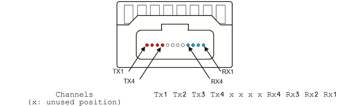
Figure 14-44: Optical receptacle and channel orientation for MPO-12 connector
