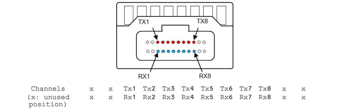
Figure 14-47: Optical receptacle and channel orientation for MPO-12 Two Row connector
