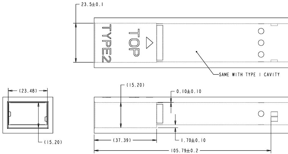
Figure 11-6: Impedance test jig for Type 2 OSFP
