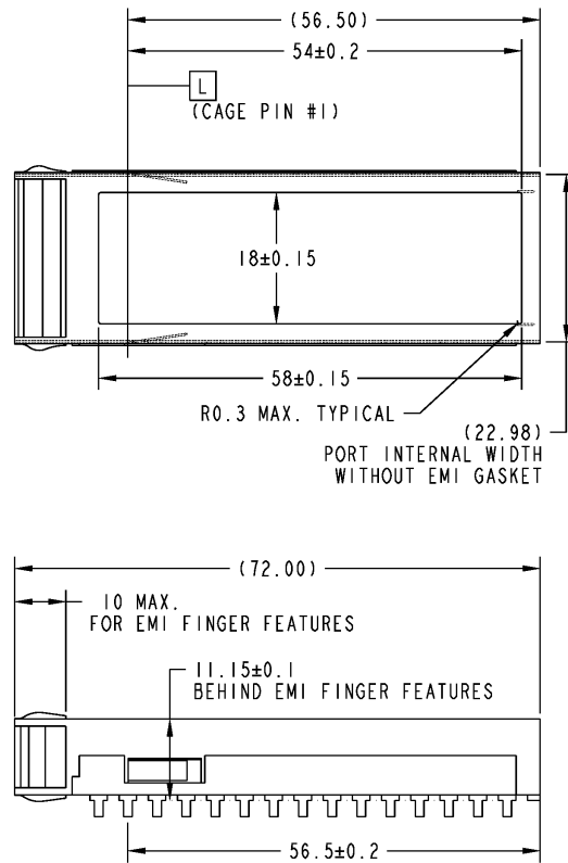
Figure 13-12: OSFP-RHS 2x1 bottom layer cage
