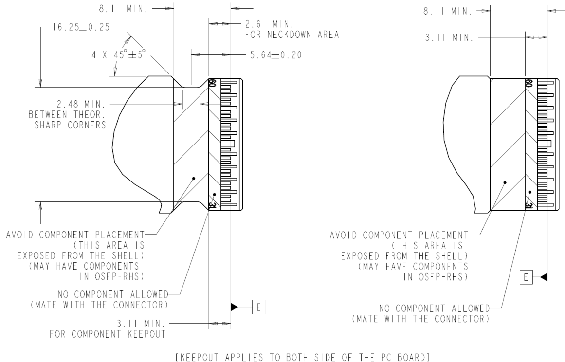
Figure 4-4: OSFP1600 module pc board (card-edge), neck area
