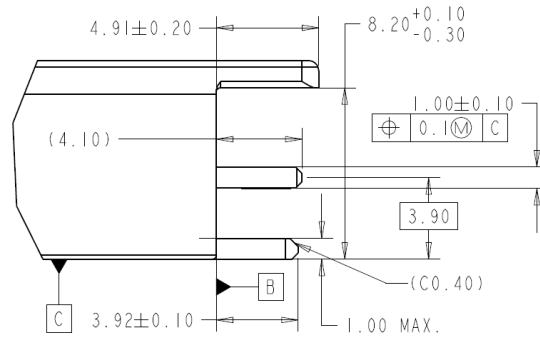
Figure 12-8: OSFP-RHS, back of the module
