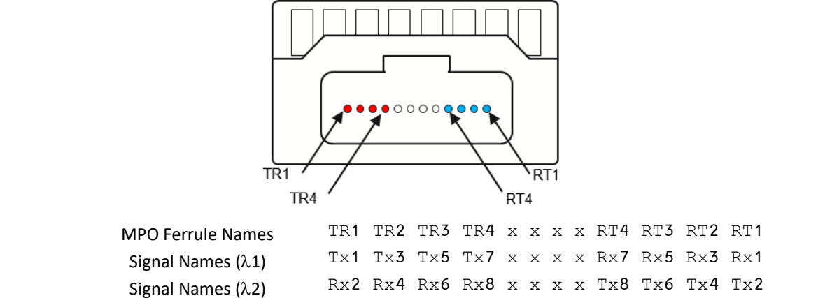
Figure 14-45: Optical receptacle and channel orientation for MPO-12 for 400G-SR4.2
