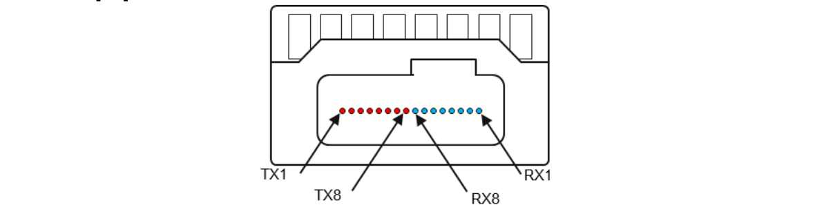
Figure 14-46: Optical receptacle and channel orientation for MPO-16 connector
