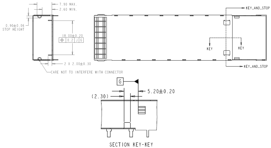
Figure 12-19: Keying feature in OSFP-RHS
