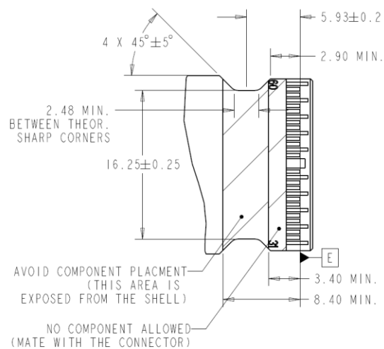
Figure 3-24: Keepout area and neck shape for OSFP
