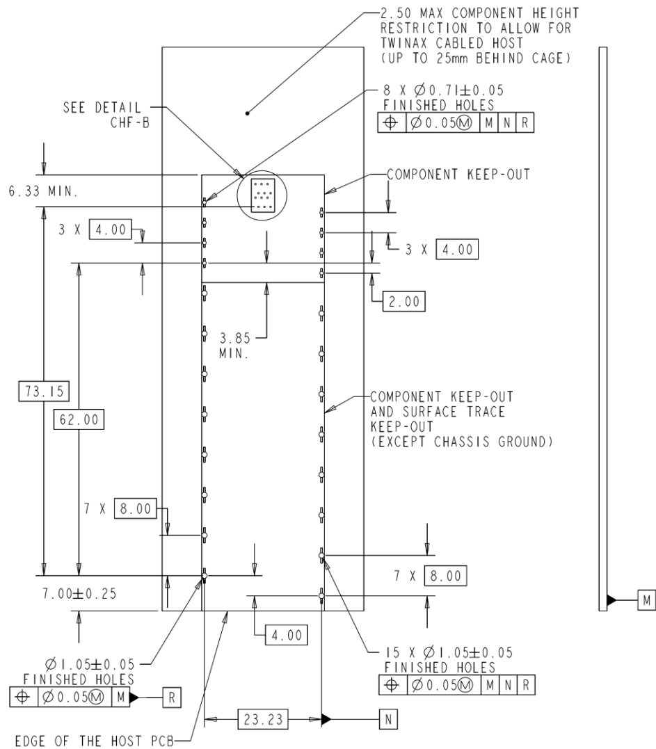
Figure 9-3: CHF-B (Cabled Host Footprint B)
