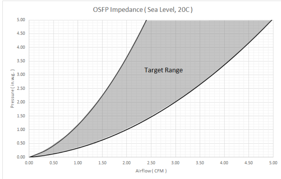
Figure 11-1: Target range of airflow impedance of an OSFP module(≤33W) (20C, Sea Level)
