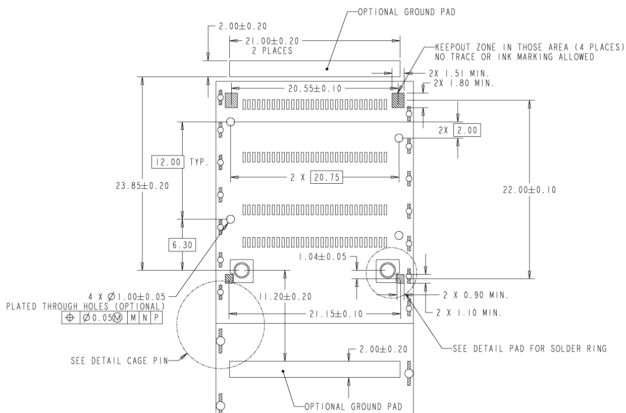
Figure 7-35: Layout for peg, retaining feature and ground pad
