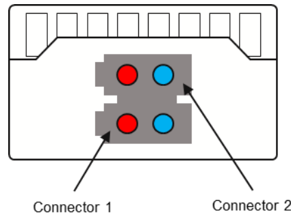
Figure 9-20: Optical receptacle for dual MDC connector (Stacked)
