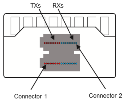
Figure 9-24: Optical receptacle for dual MMC connector (Stacked)
