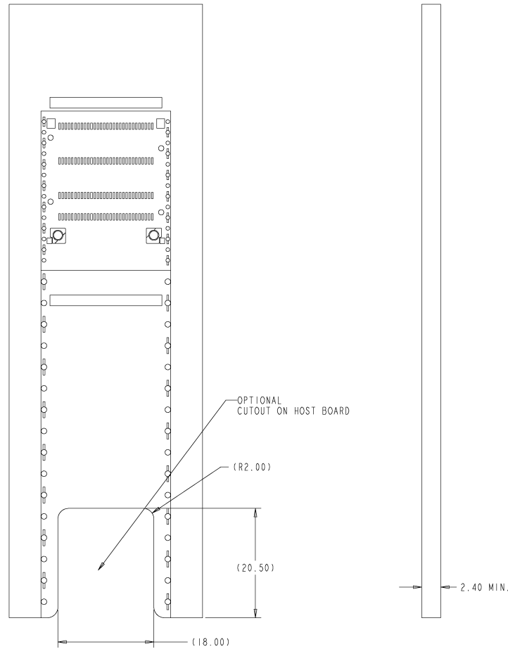
Figure 4-19: Belly to Belly 1x1 SMT PCB layout
