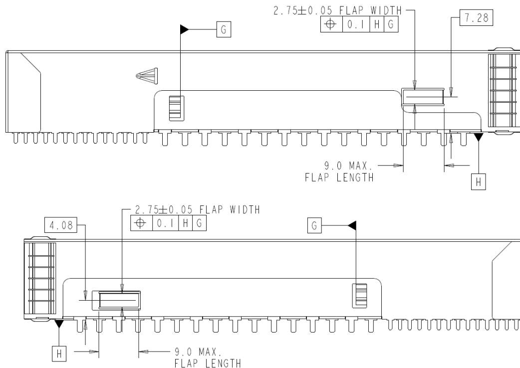
Figure 4-22: Latch feature, left and right side
