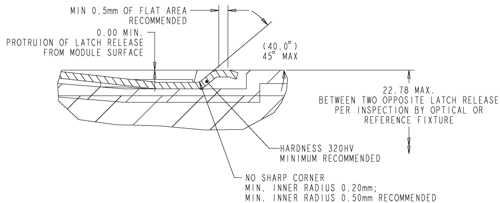
Figure 3-40: Latch plane corner radius and release details
