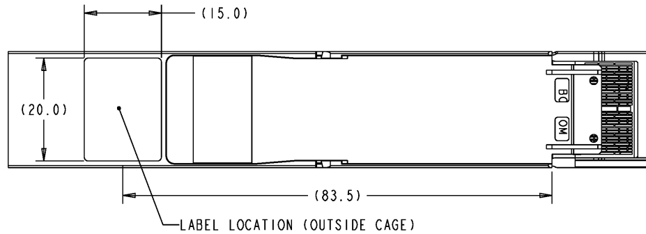
Figure 3-32: OSFP-XD, preferred label location
