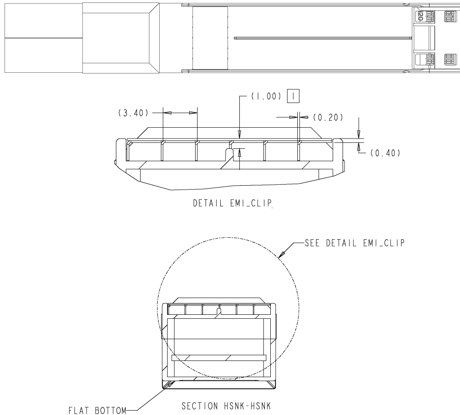
Figure 3-24: Heat sink, EMI clip airflow channel
