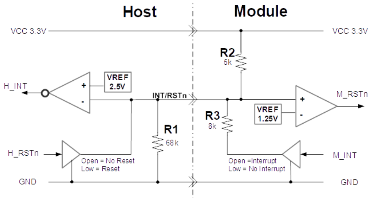
Figure 10-3: INT/RSTn circuit
