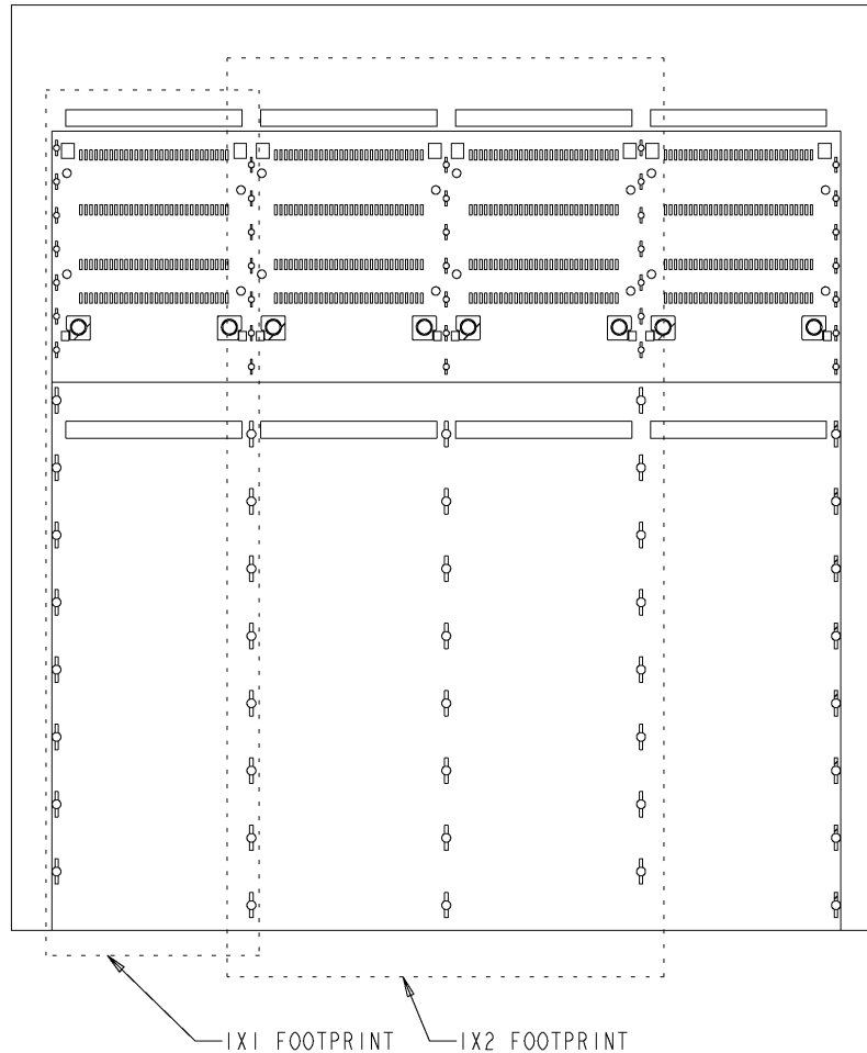
Figure 4-20: Comparison of host PCB layout between 1x1, 1x2 and 1x4
