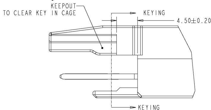
Figure 3-17: OSFP-XD, Keying feature length
