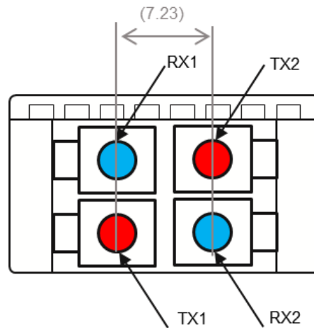
Figure 9-16: Optical receptacle and channel orientation for Dual LC
