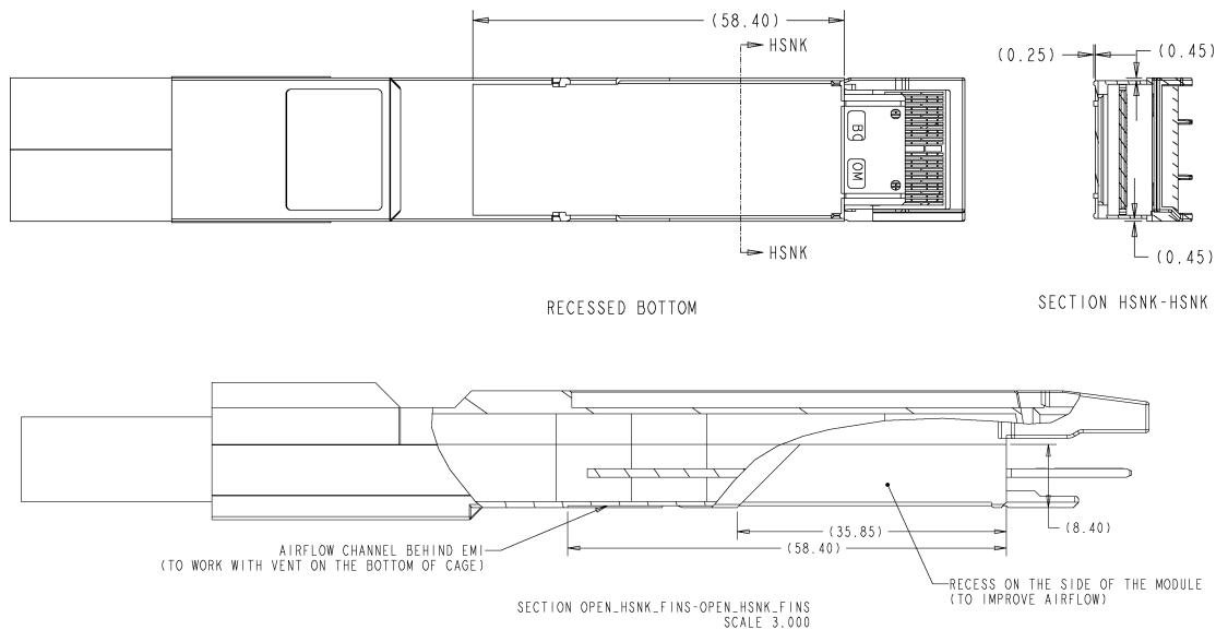
Figure 3-31: OSFP-XD, recessed bottom
