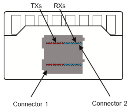
Figure 9-26: Optical receptacle for dual SN-MT connector (Stacked)
