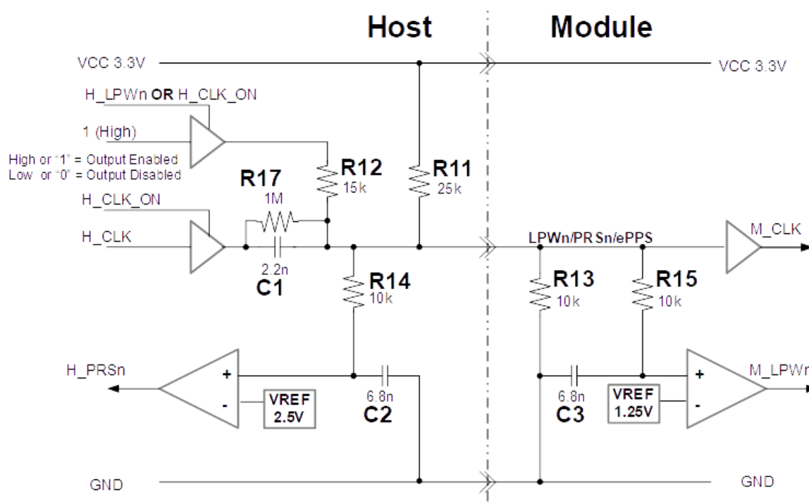
Figure 10-6: LPWn/PRSn/ePPS circuit
