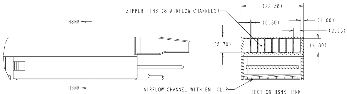
Figure 3-20: Heatsink, Zipper fin
