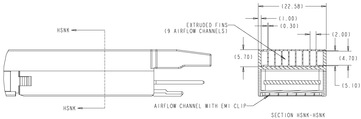
Figure 3-21: Heatsink, Aluminum Extrusion
