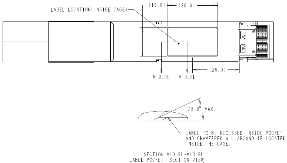
Figure 3-33: OSFP-XD, optional label location
