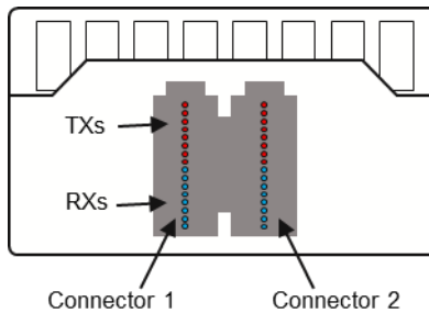
Figure 9-23: Optical receptacle for dual MMC connector (Ganged)
