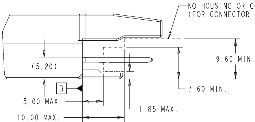
Figure 3-10: OSFP-XD, no component area
