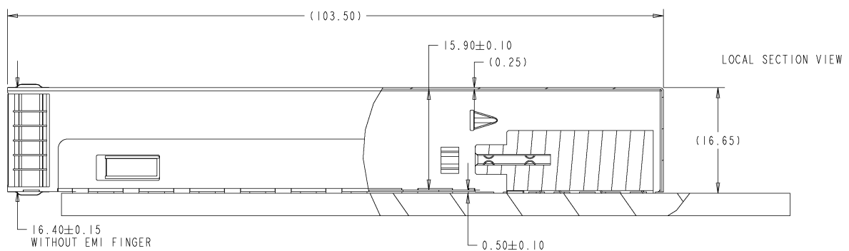
Figure 4-5: Side view of a 1x1 cage with vertical cage dimensions
