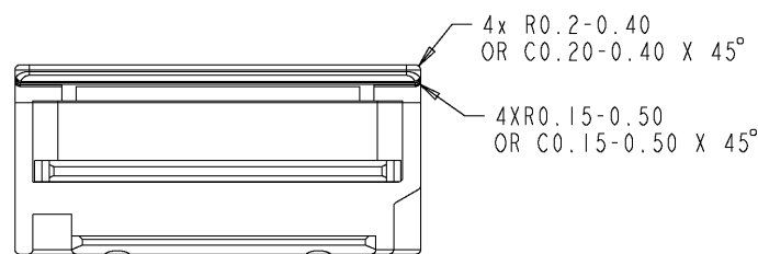
Figure 8-4: Corner radius of OSFP-XD-RHS in back view
