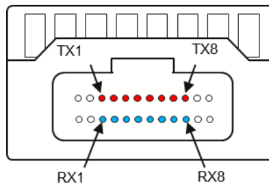
Figure 9-12: Optical receptacle and channel orientation for MPO-12 Two Row connector
