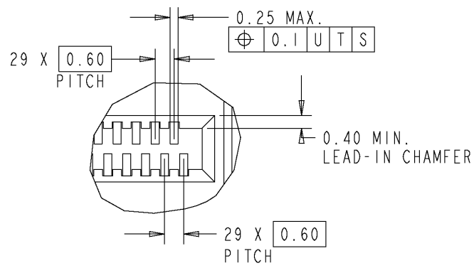
DETAIL CONTACT
