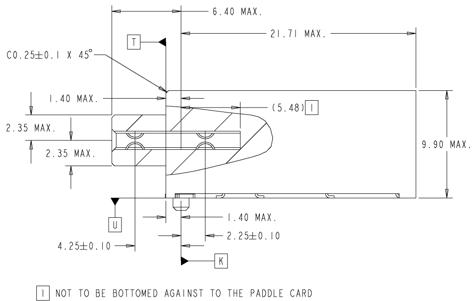
Figure 4-28: Surface mount connector, detail contact
