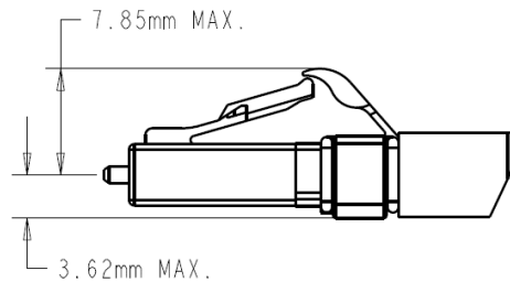
Figure 9-17: LC connector size requirement per given belly-to-belly pitch
