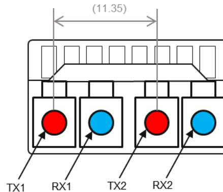
Figure 9-15: Optical receptacle and channel orientation for Dual Mini-LC
