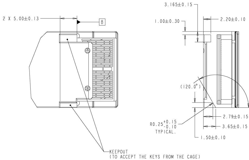
Figure 8-11: Keying feature
