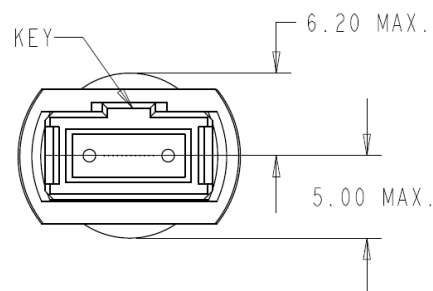
Figure 9-30: MPO connector size requirement per given belly-to-belly pitch
