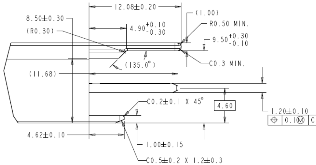
Figure 8-7: OSFP-XD-RHS, back of the module
