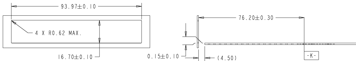
Figure 4-26: Bezel design for 1x4 cage
