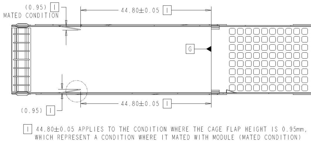
Figure 4-24: Latch flap, dimension from the positive stop
