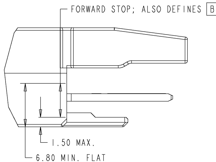
Figure 3-11: OSFP-XD, location of the forward stop
