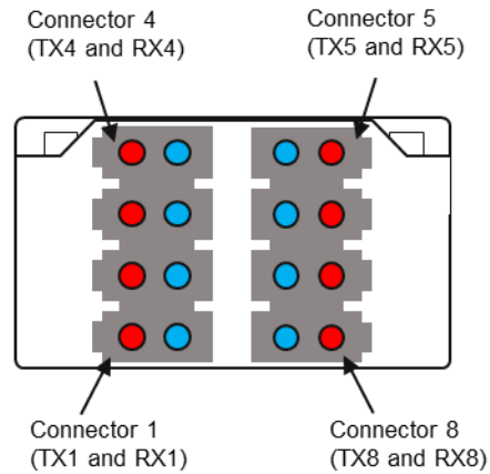
Figure 9-31: Optical receptacle and channel orientation for 8 x MDC connector
