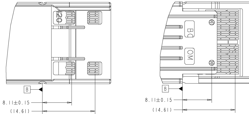
Figure 3-14: Signal pad location to module (left: top view, right: bottom view)
