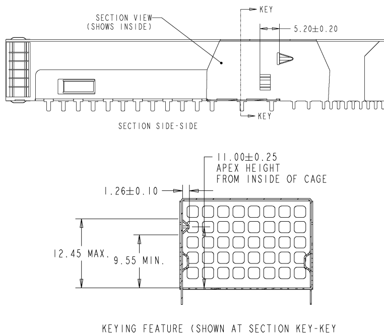
Figure 4-12: Cage Keying feature
