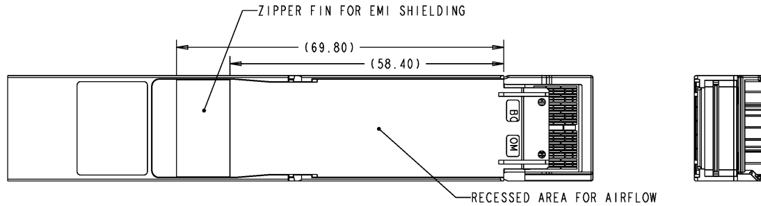
Figure 3-30: OSFP-XD, EMI clip bottom
