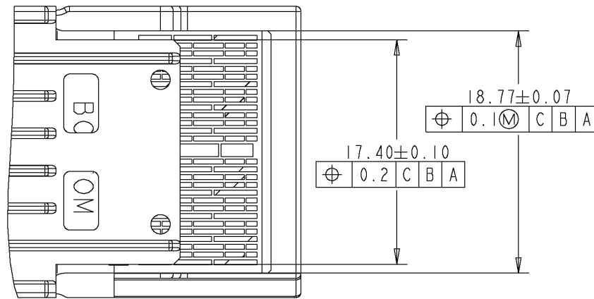
Figure 3-8: OSFP-XD, back, in the bottom view
