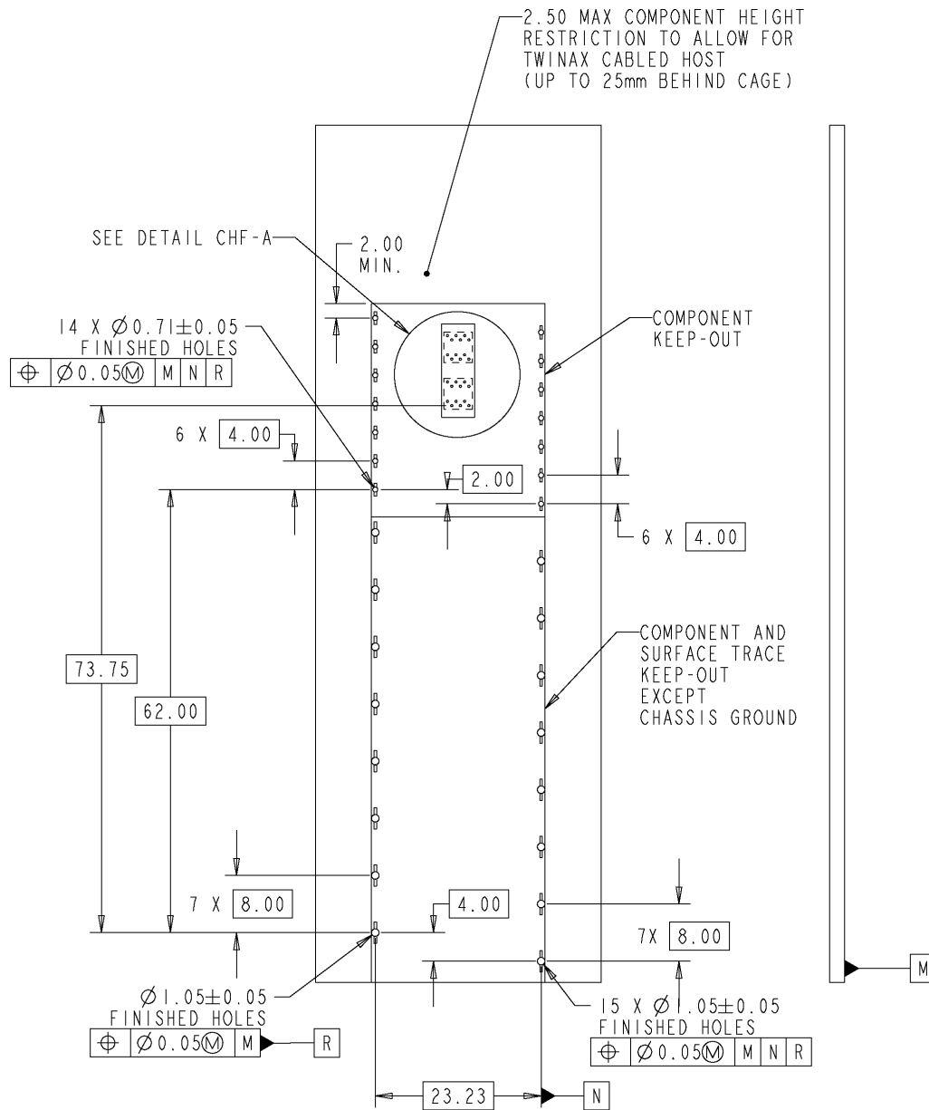
Figure 5-1: CHF-A (Cabled Host Footprint A)
