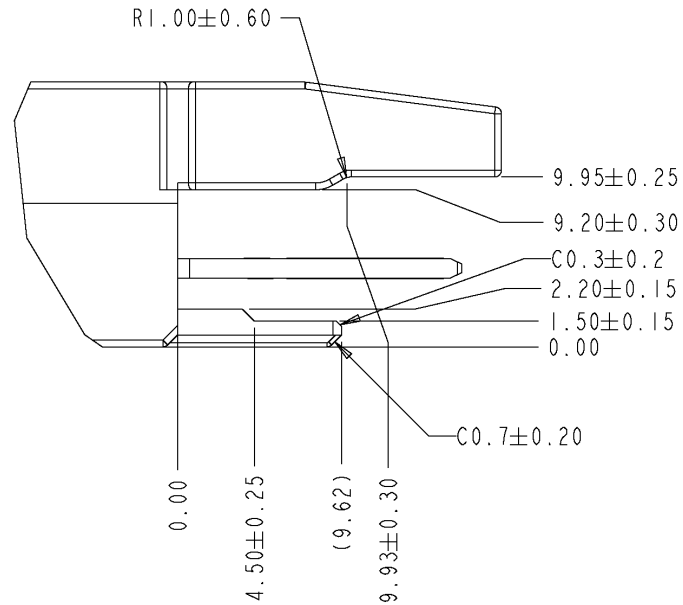
Figure 3-7: OSFP-XD, structure shape
