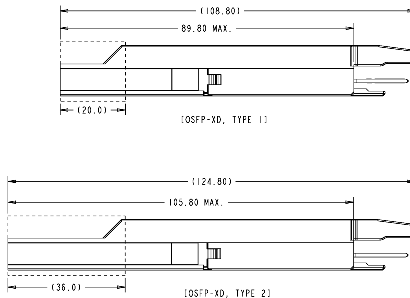
Figure 3-3: OSFP-XD type 1 and 2 (module length)
