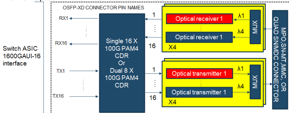
Figure 9-5: Block diagram for 1600G 4FR4
