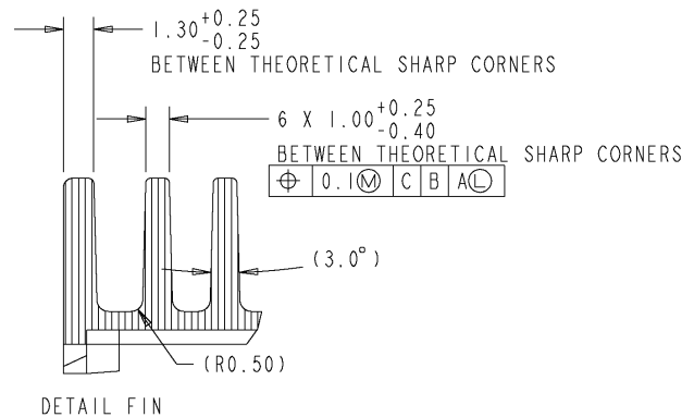
Figure 3-23: Heat sink, Open top, Detail Fin
