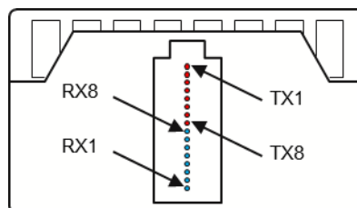
Figure 9-13: Optical receptacle and channel orientation for MXC connector
