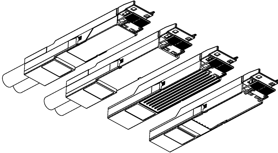
Figure 3-27: OSFP-XD, various bottom shape
