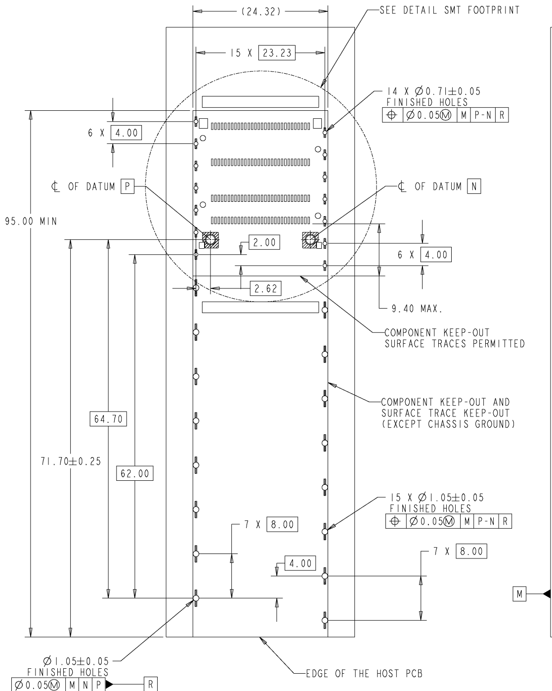
Figure 4-16: Host PCB layout for 1x1 cage
