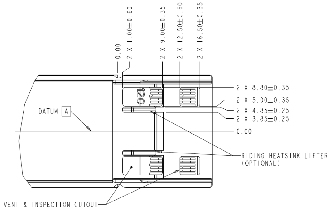
Figure 3-12: OSFP-XD, dimension for ventilation holes
