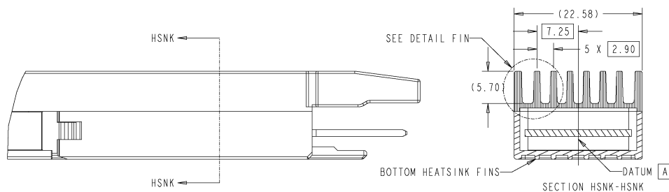
Figure 3-22: Heatsink, Open Top
