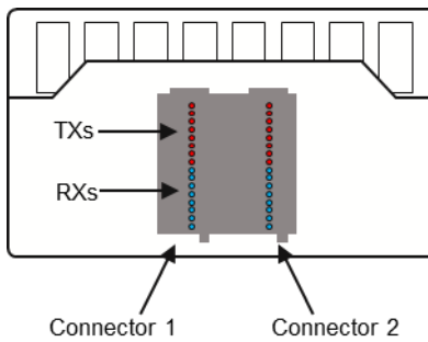
Figure 9-25: Optical receptacle for dual SN-MT connector (Ganged)
