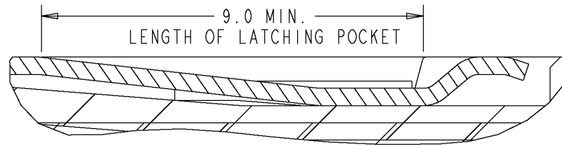
Figure 3-39: Latching pocket length
