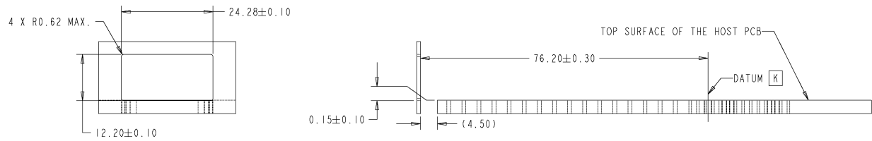
Figure 8-24: Bezel cutout for the OSFP-XD-RHS cage
