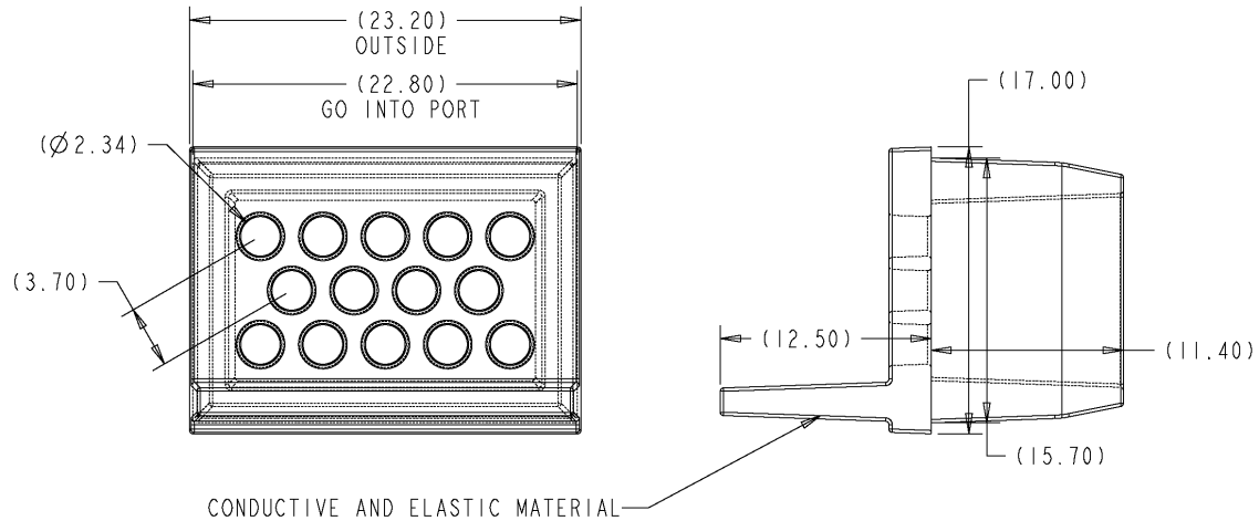
Figure 4-30: OSFP-XD blank plug (reference design)
