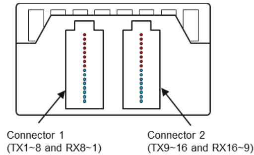
Figure 9-14: Optical receptacle and channel orientation for Dual MXC connector
