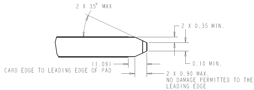
Figure 3-35: OSFP-XD card-edge, detail chamfer (lead-in chamfer)
