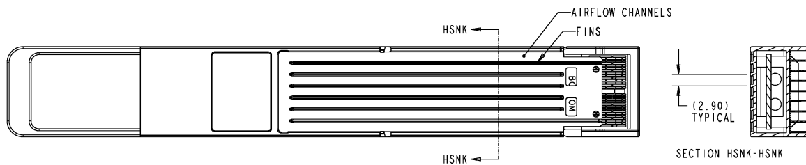
Figure 3-29: OSFP-XD, Bottom heatsink fins
