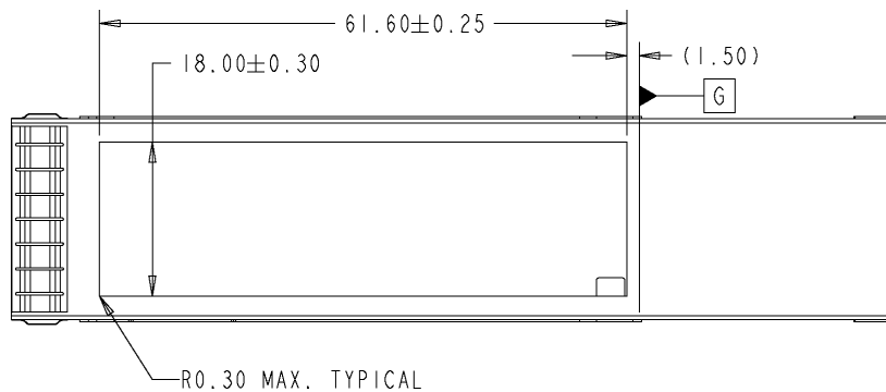
Figure 8-23: Cutout for a riding heat sink in the OSFP-XD-RHS cage
