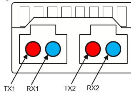
Figure 9-18: Optical receptacle and channel orientation for dual CS® connector
