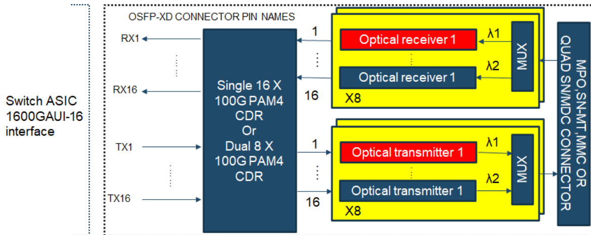
Figure 9-3: Block diagram for 1600G 4FR2
