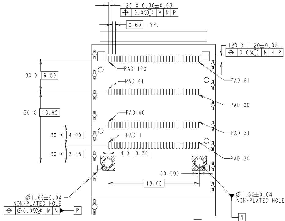
Figure 4-17: Host PCB layout, details
