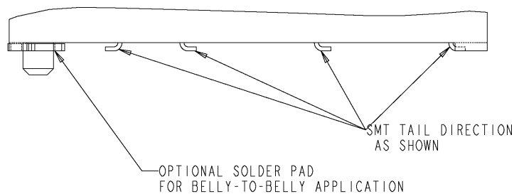
Figure 4-29: Surface mount connector, from the side view
