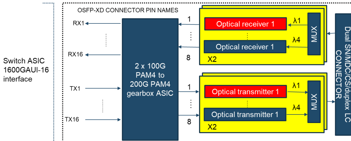
Figure 9-6: Block diagram for 1600G 2FR4
