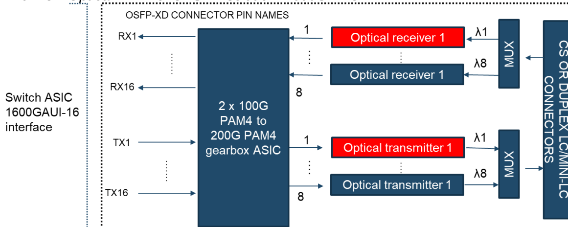
Figure 9-8: Block diagram for 1600G FR8
