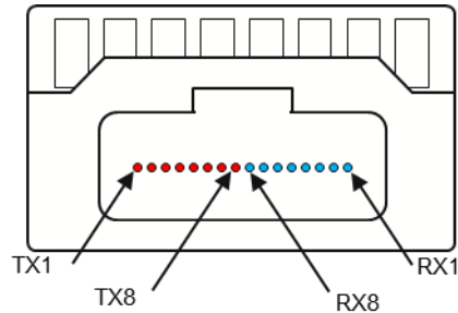
Figure 9-11: Optical receptacle and channel orientation for MPO-16 connector
