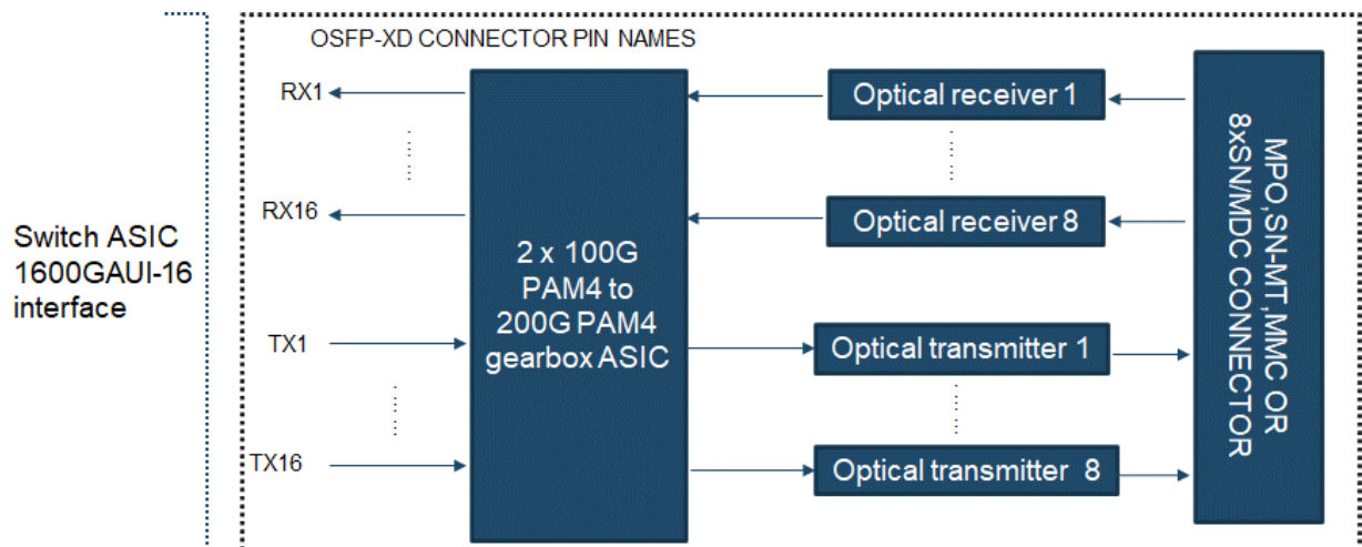
Figure 9-2: Block diagram for 1600G DR8
