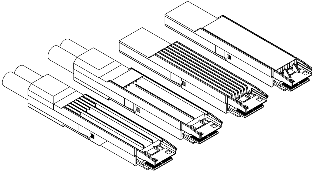
Figure 3-19: OSFP-XD, various heatsink shape
