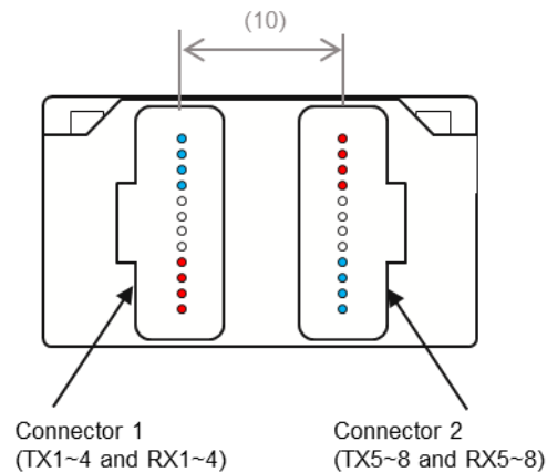
Figure 9-29: Optical receptacle and channel orientation for Dual MPO connector
