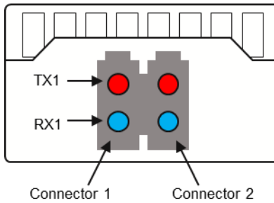
Figure 9-19: Optical receptacle for dual MDC connector (ganged)
