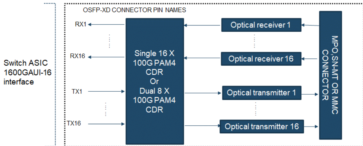
Figure 9-1: Block diagram for 1600G DR16
