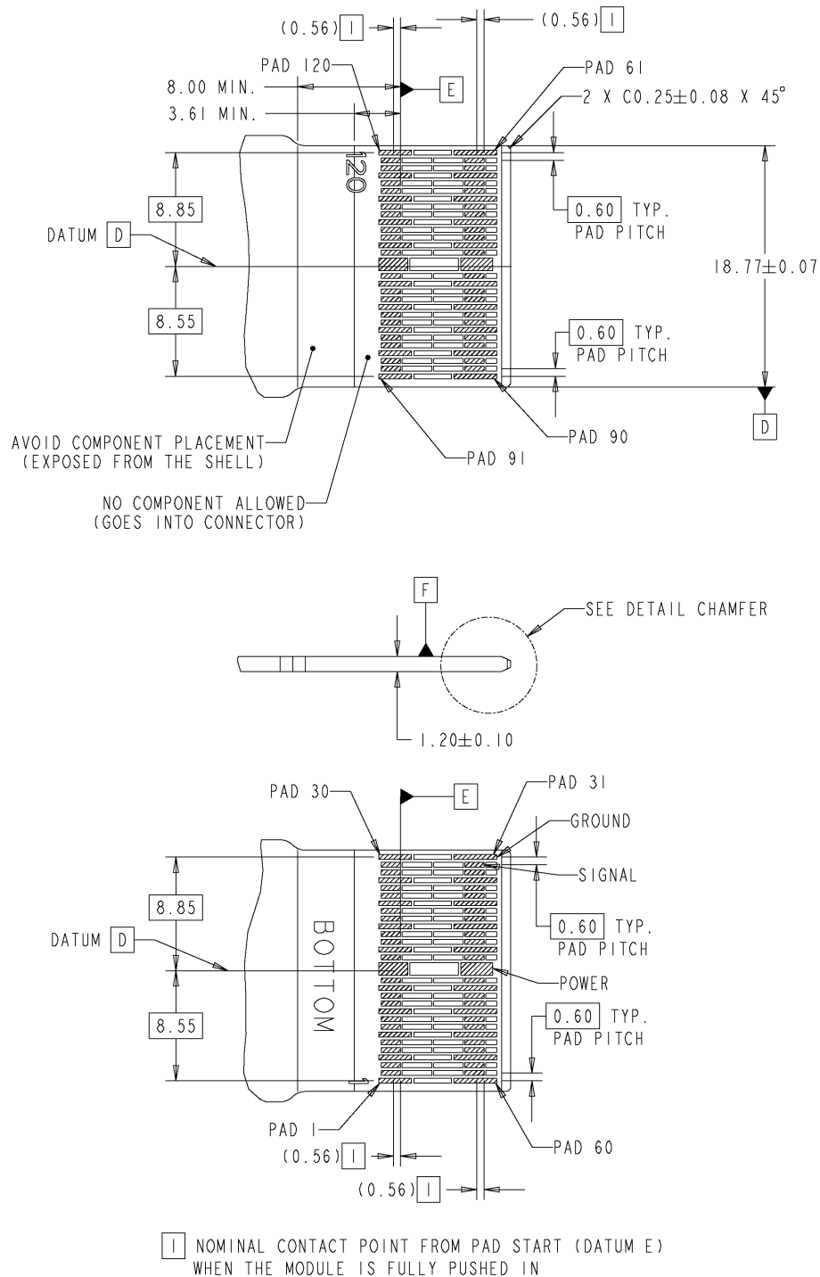
Figure 3-34: OSFP-XD module pc board (card-edge)
