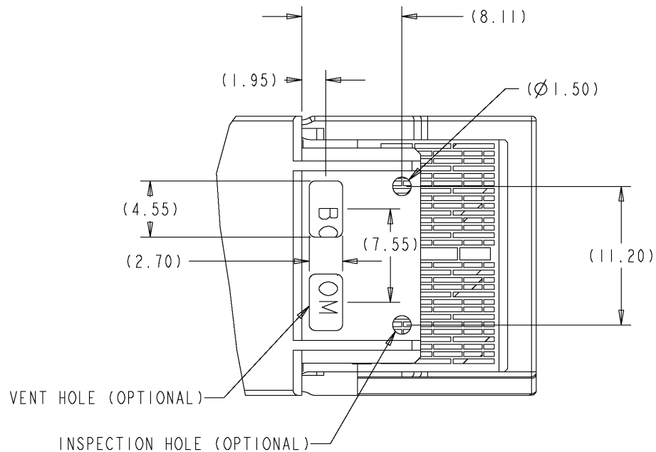
Figure 3-9: OSFP-XD, optional signal pad inspection holes
