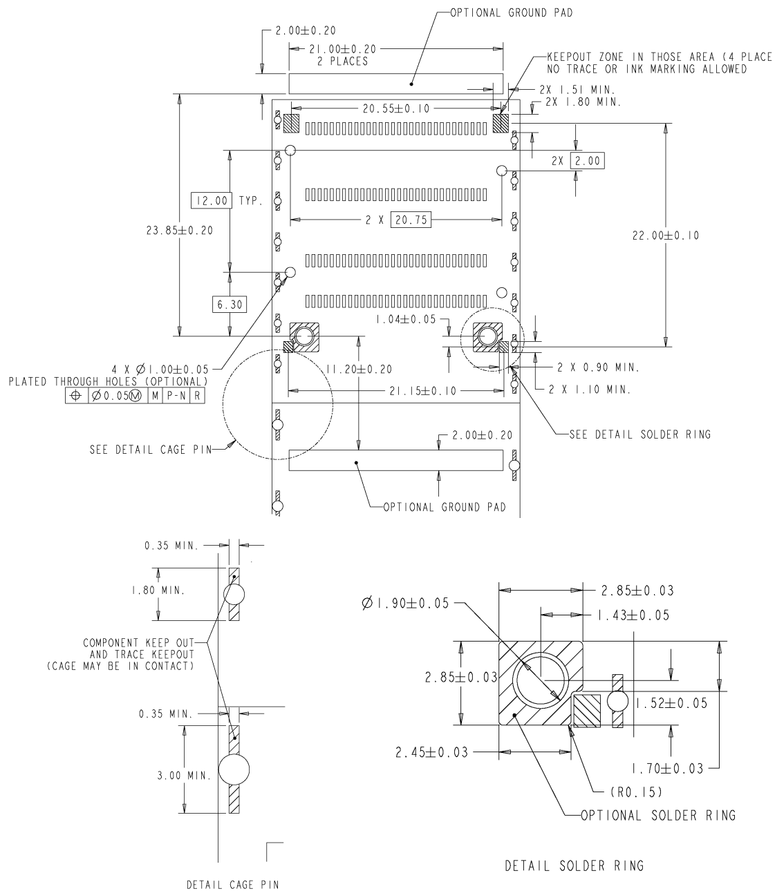
Figure 4-18: Solder ring and cage touchdown keepout
