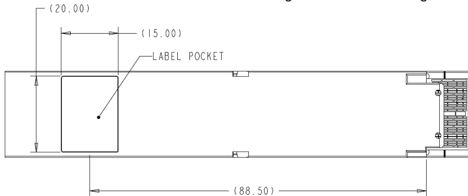
Figure 8-12: Label location (preferred)
