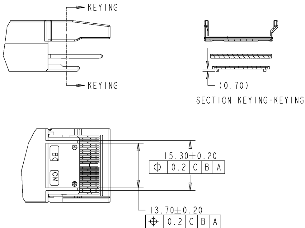
Figure 3-15: Bottom ribs
