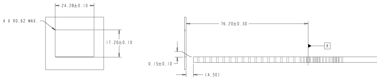
Figure 4-25: Bezel design and location for 1x1 cage
