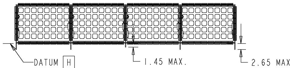
Figure 4-21: Compliance pin length, 1x4 Cage
