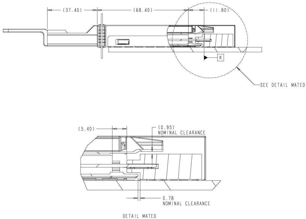
Figure 4-6: Side view of a 1x1 cage with axial reference dimensions
