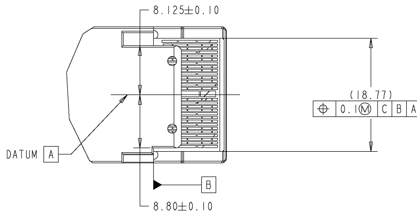
Figure 8-8: Paddle card position (bottom view of module) and module width
