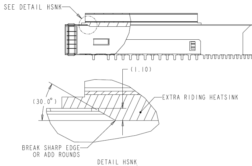
Figure 4-14: Cutout on the cage for a riding heatsink
