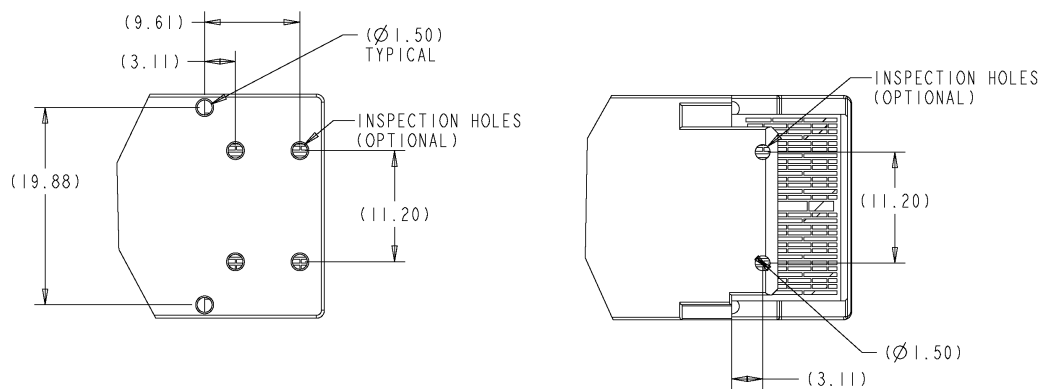
Figure 8-9: Location of inspection holes
