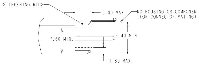
Figure 8-6: Connector keep out area from the side view
