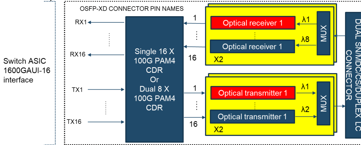
Figure 9-7: Block diagram for 1600G 2FR8
