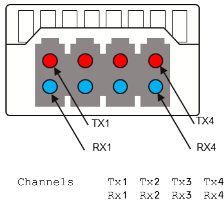
Figure 9-27: Optical receptacle and channel orientation for quad MDC connector
