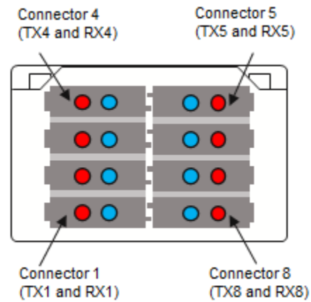
Figure 9-32: Optical receptacle and channel orientation for 8 x SN ® connector
