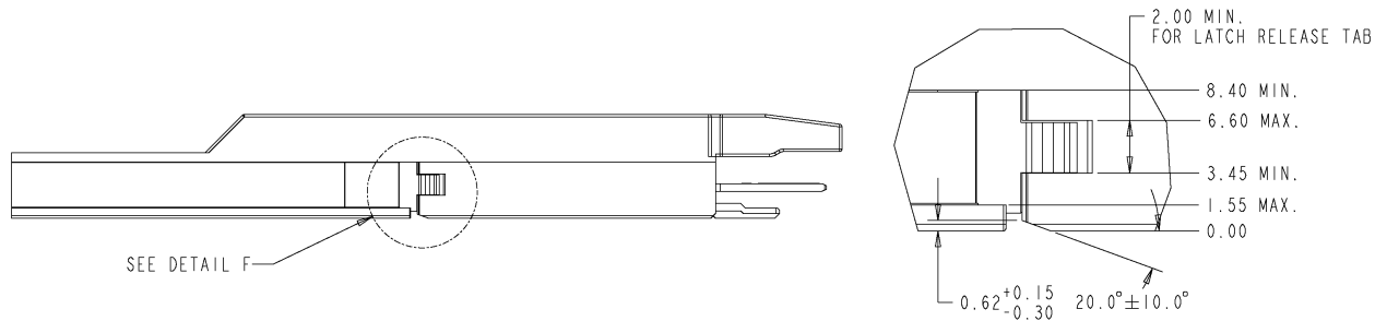
Figure 3-37: Latch pocket location
