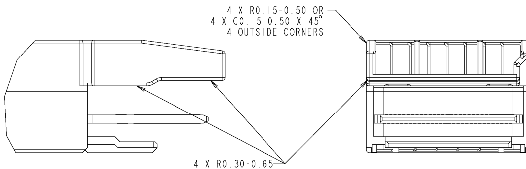
Figure 3-5: OSFP-XD corner radius
