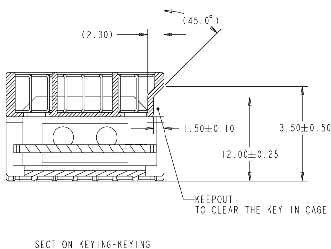
Figure 3-18: OSFP-XD, keying feature height (section view)
