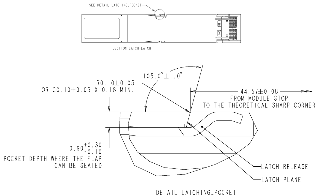
Figure 3-38: Latch release max width and latching pocket round
