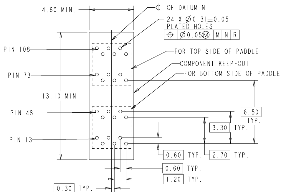
DETAIL CHF-A
