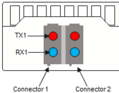
Figure 9-21: Optical receptacle for dual SN connector (ganged)
