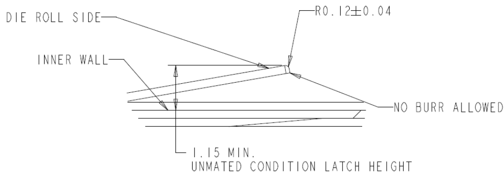
Figure 4-23: Latch flap, cross-sectional view from top
