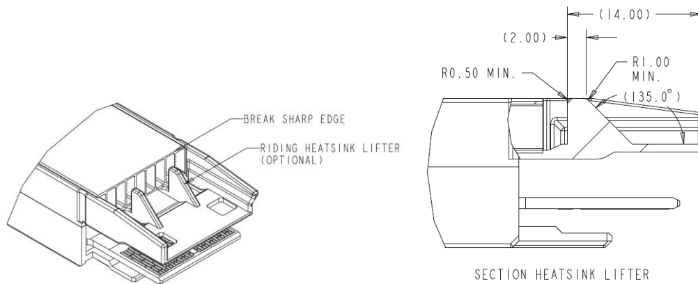
Figure 3-16: Heatsink lifter
